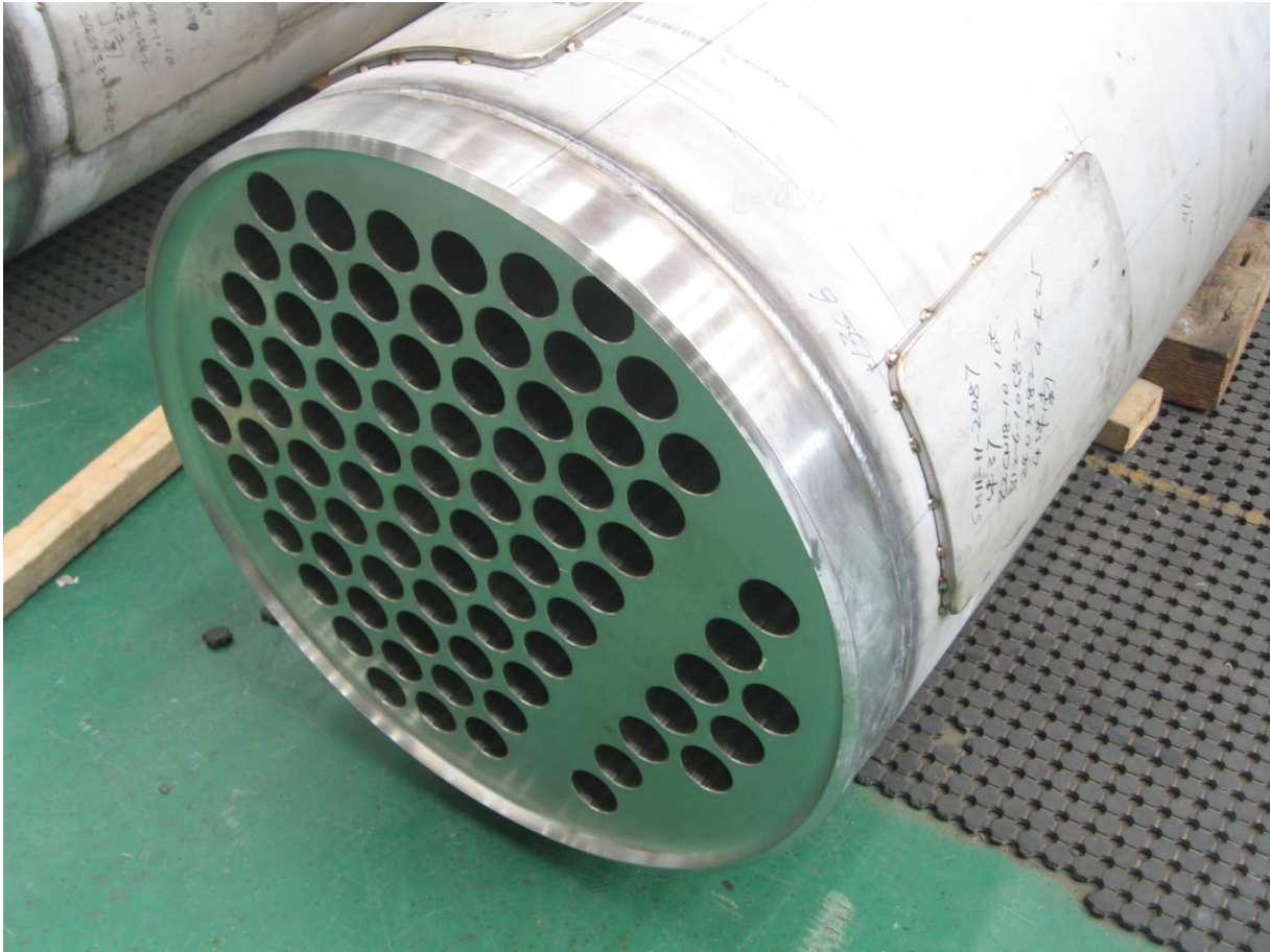
Manufacturing supervision - Shells of heat exchangers at SMPV Morimatsu Shanghai (China)
