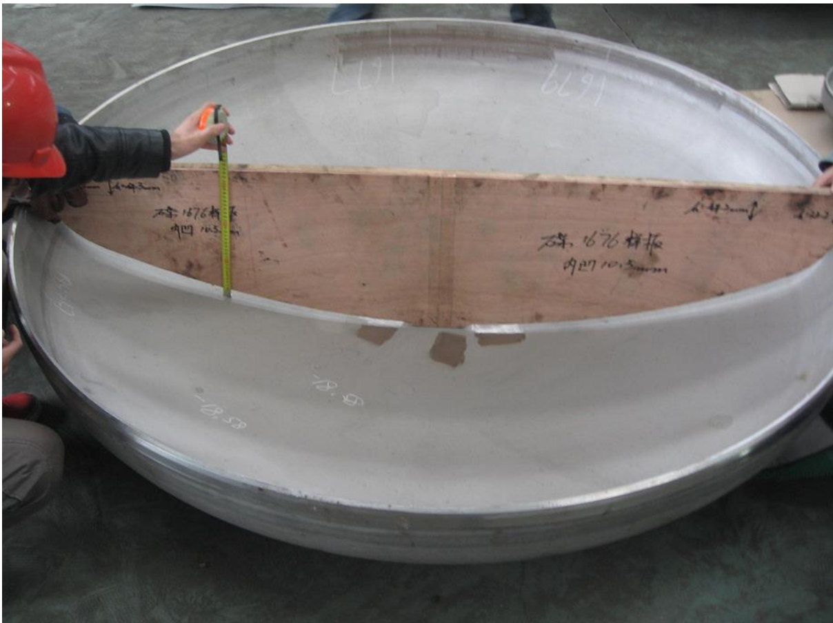
Procurement inspection – Dish heads final inspection at Qiangzhou Xitang Wuxi (China)
