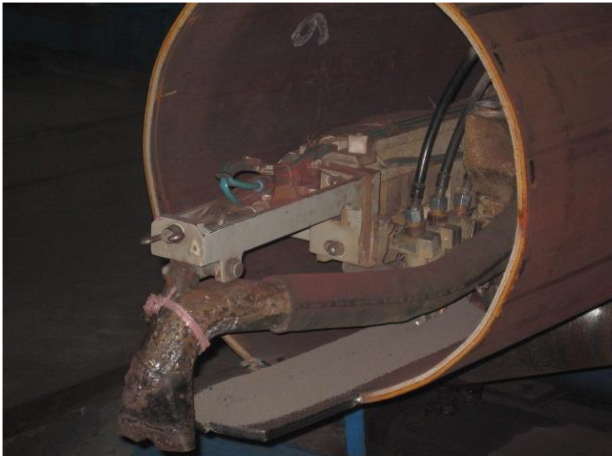
Technical Audit of Essar Pipings at Hazira (India) for SAW welded tubes
