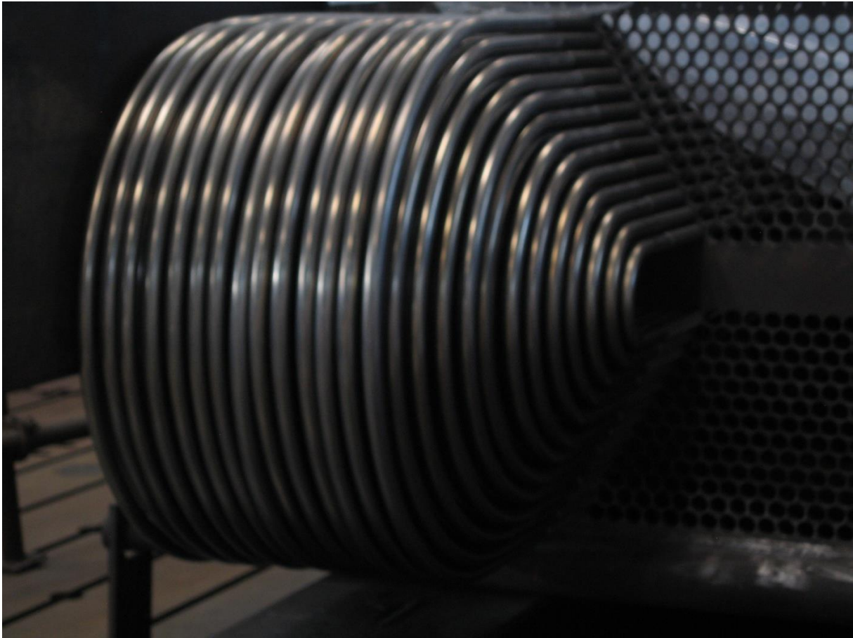
Manufacturing inspection - Superheater of the MSR at Dong Fang Heavy Manufacturing Nansha (China)
